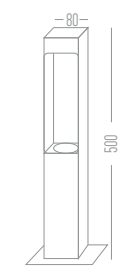
Torch 50 ● ● GU 10 x 1 220 V 50 W IP55 Price : 4.900 Baht
